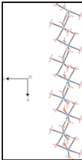
Fig. 2. Polymeric chain of sodium cations and water molecules, viewed along [1\ 0\ 0] .
